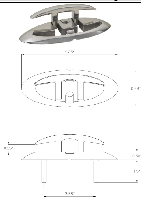
#93.451 Oval fold down cleat 4.5 inch Stud Mount
