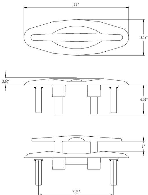
#93.305 Pop up Cleat; Foot print: 11 inch x 3.5 inch. (Wide line 305). Spring Loaded. Pops up by pushing button. Finish: Polished Stainless Steel;
