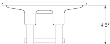
93.102T - 15 inch Pop up Cleat; Top[ Mounted with visible screw holes (202-6) Foot print: 17 inch x 3.4 inch. Finish: Polished Stainless Steel;
