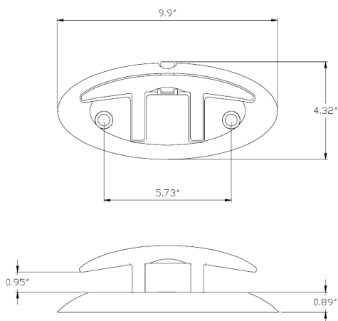
#93.600 Oval fold down cleat 6 inch Top Mount
