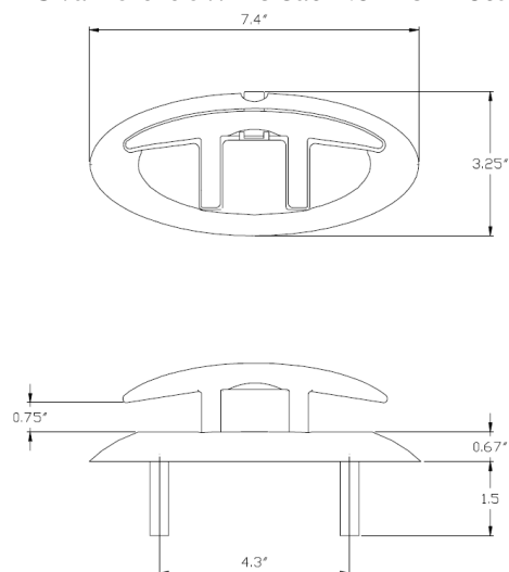
#93.601 Oval fold down cleat 6 inch Stud Mount
