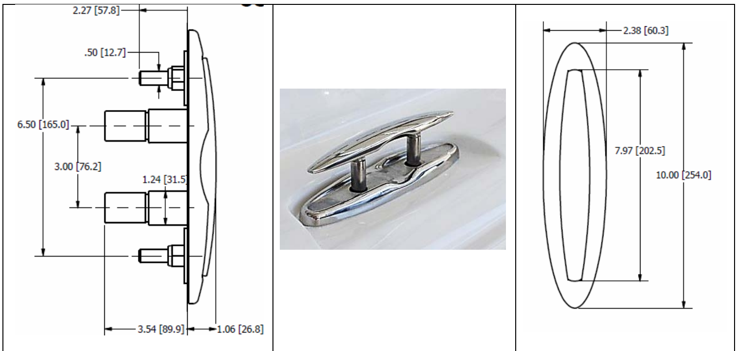
#93.104 Pop up Cleat; 10 inch x 2.38 inch. Surface Mount.
