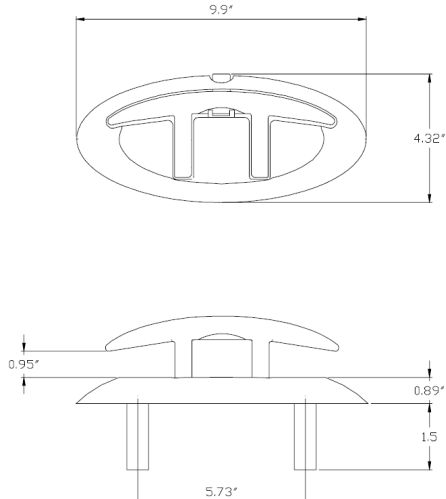
#93.801 Oval fold down cleat 8 inch Stud Mount
