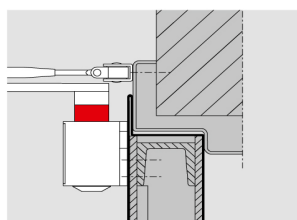
Closer body TS 83
