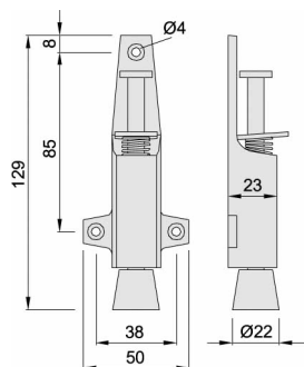
#32.021.003 Door holder, Push type Throw: 25 mm ALUMINUM ANODIZED - Seawater resistant
