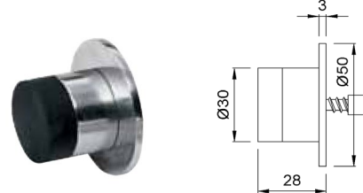
32.009.508 door stop 30 mm or 1 3/16" long.
