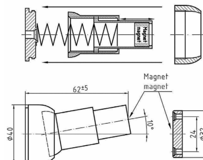
Magnetic doorholder #34.410B.266 Polished chrome finish spring loaded, swivel; Light duty for light weight doors
