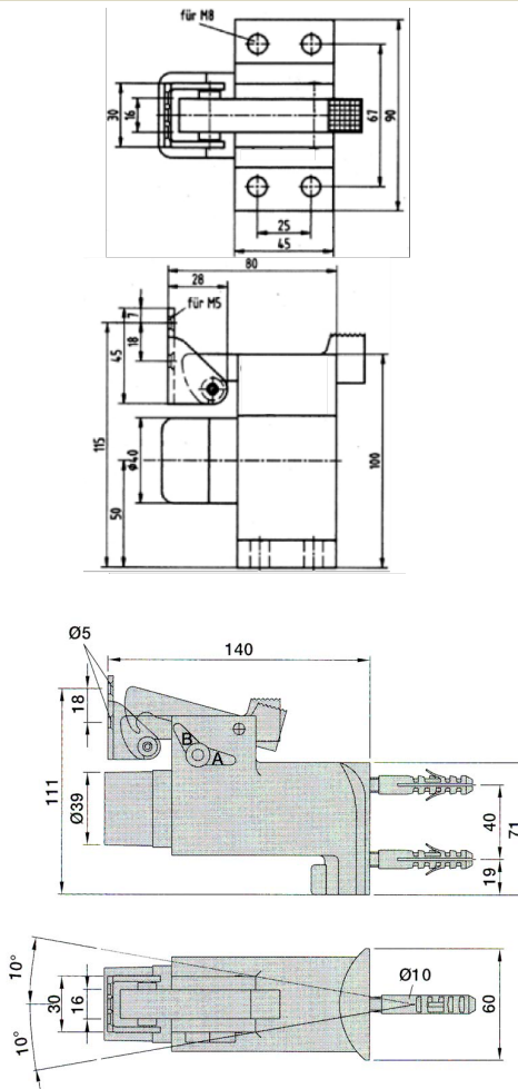
#32.010.003 Spring loaded hook type door holder.
