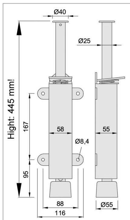
32.1043.101 Doorholder 120 mm ~ 4.75" throw STEEL LAQUERED - MAX DOOR WEIGHT 200 KG COMMERCIAL GRADE
