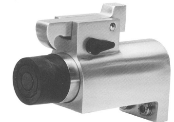
#32.1012.003 Spring loaded hook type door holder. Rigid wall mounted.
