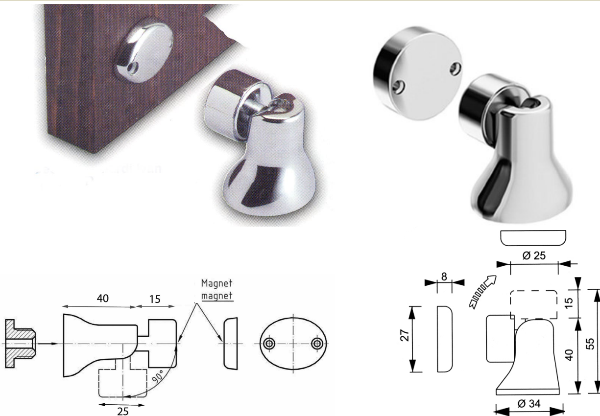
Magnetic doorholder #34.252.266 Polished Chrome Finish; Light duty for light weight doors Magnetic doorholder #34.252.566 Satin Chrome Finish; Light duty for light weight doors Magnetic doorholder #34.252.106 Polished Brass Finish; Light duty for light weight doors
