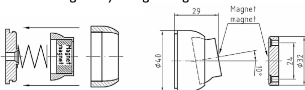
Magnetic doorholder #34.410S.266 Polished chrome finish spring loaded, swivel; Light duty for light weight doors
