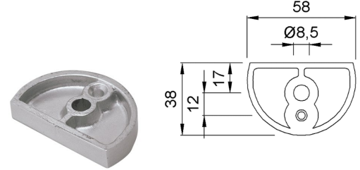
#32.558 Shim 10 mm high Black Aluminum
