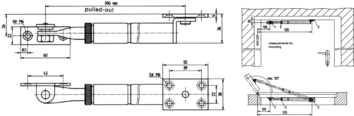
#32.017.508 Telescopic Doorstay, stainless steel, with brake. Heavy duty up to 150 lbs. door weight Travel: 200 mm or 8".
