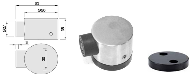
#32.111 doorbuffer 32.101 filler plate 3/8"
