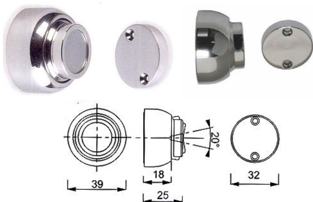
Magnetic doorholder #34.410S.266 Polished chrome finish spring loaded, swivel; Light duty for light weight doors
