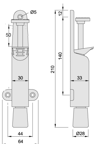
#32.029.106 Doorholder 50 mm ~ 2" throw
