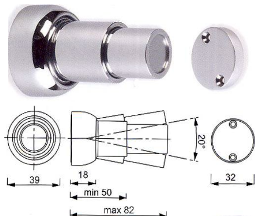
Magnetic doorholder #34.410B.266 Polished chrome finish spring loaded, swivel; Light duty for light weight doors
