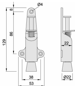
#32.024.106 Door holder, Push type Throw: 25 mm
