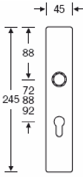
#12.1410
