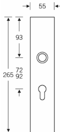
#12.1433F
