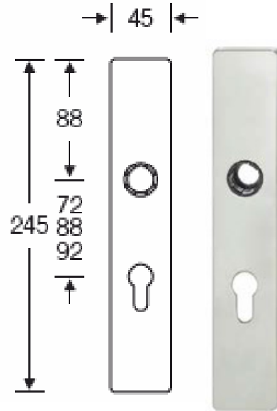
#12.1410
