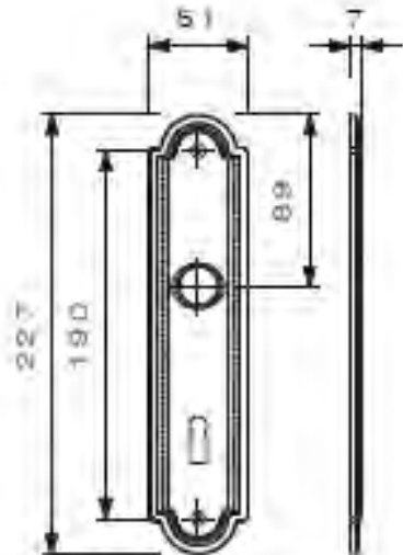
Set: with escutcheon plate #13.J336
