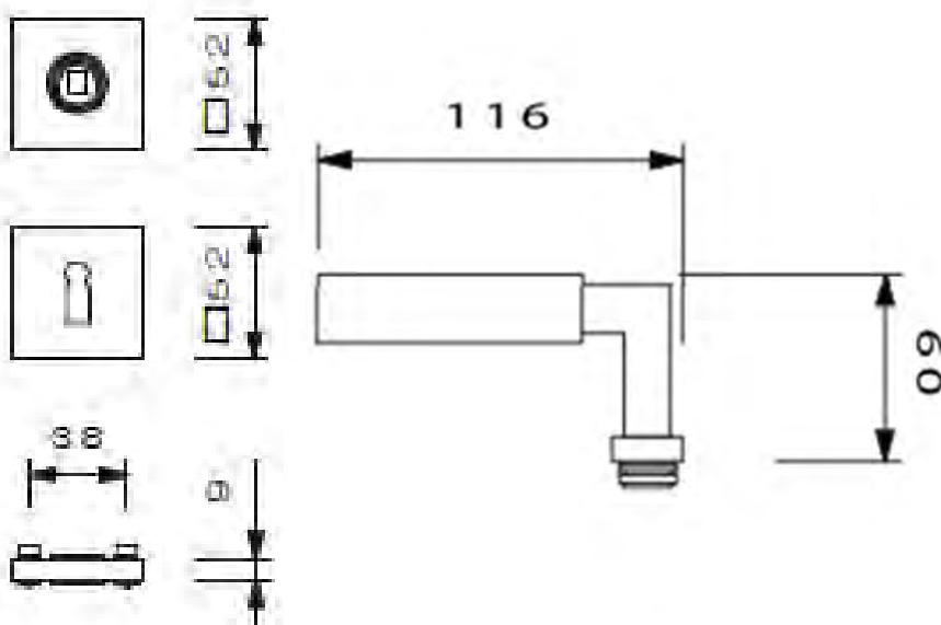
LEVER #14.J3402 "BAUHAUS" ENTRY SET DEPICTED Satin nickel plated brass
