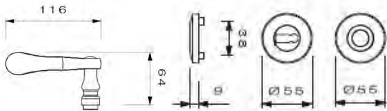
LEVER #13.J9015 "SCHONBRUNN" ESCUTCHEON #13.J51
