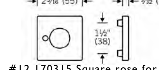
#12.170315 Square rose for tubular privacy latch; 55 x 55 mm
