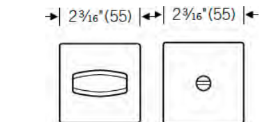
Privacy set With square roses flat 55 x 55 mm
