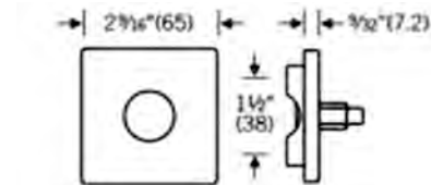
Stainless steel rose square, pair 65 x 65 mm or 2 9/16 inch Clip on style with inner rose Screws invisible
