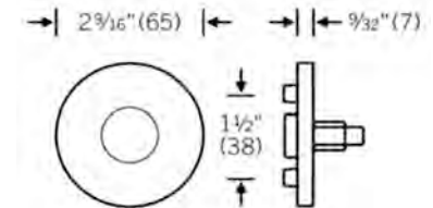
Stainless steel rose round, 65 mm or 2 9/16 inch diameter Clip on style with inner rose Screws invisible
