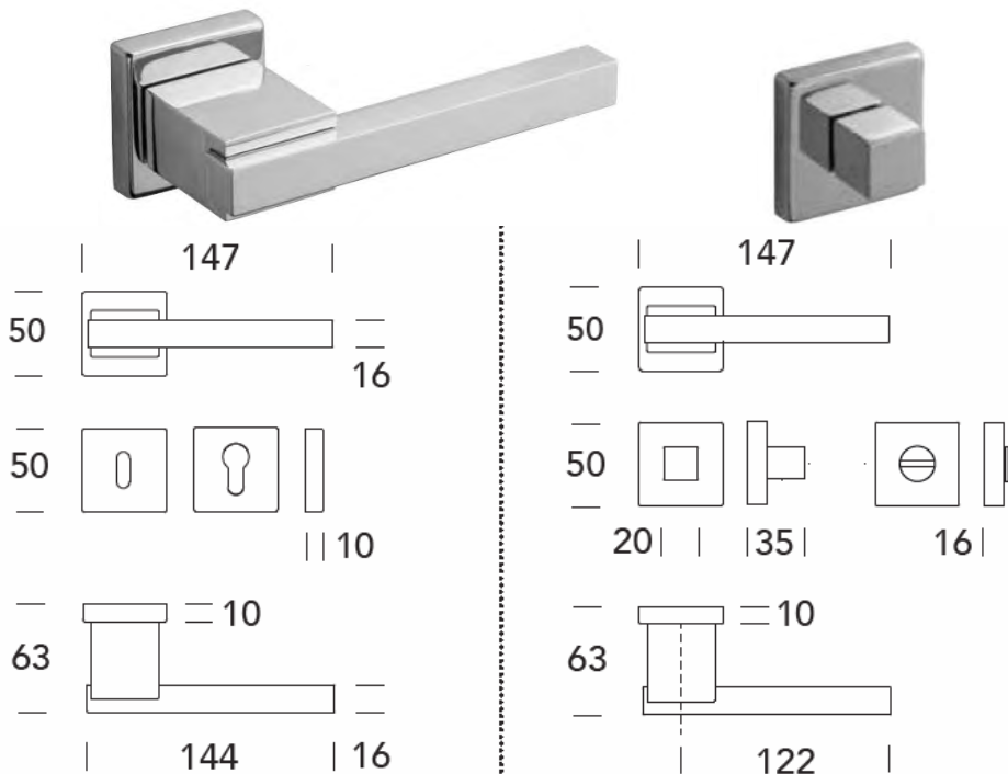
With square rose 50x50 mm; all functions available
