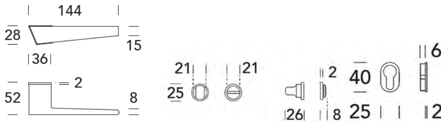
Minimal Cylinder Key Rose and Privacy thumb-turn- indicator
