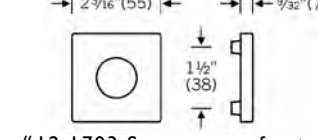
#12.1703 Square rose for tubular latch 55 x 55 mm
