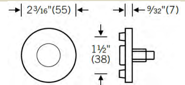
Stainless steel rose round, 55 mm or 2 3/16 inch diameter Clip on style with inner rose Screws invisible
