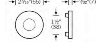
#12.173114 Rose for tubular latch
