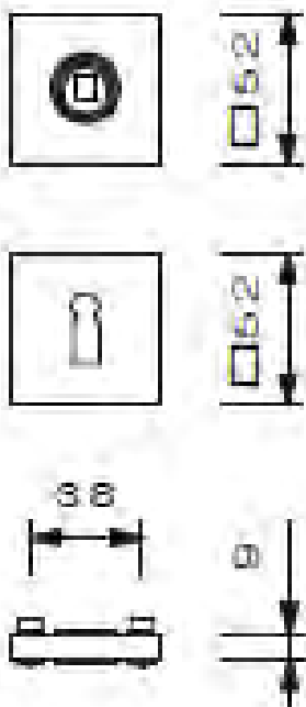
Rose 14.R3711; 52 x 52 mm x 9 mm Polished Chrome
