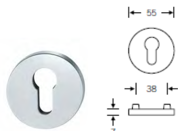
Key Rose #12.111.Z508
