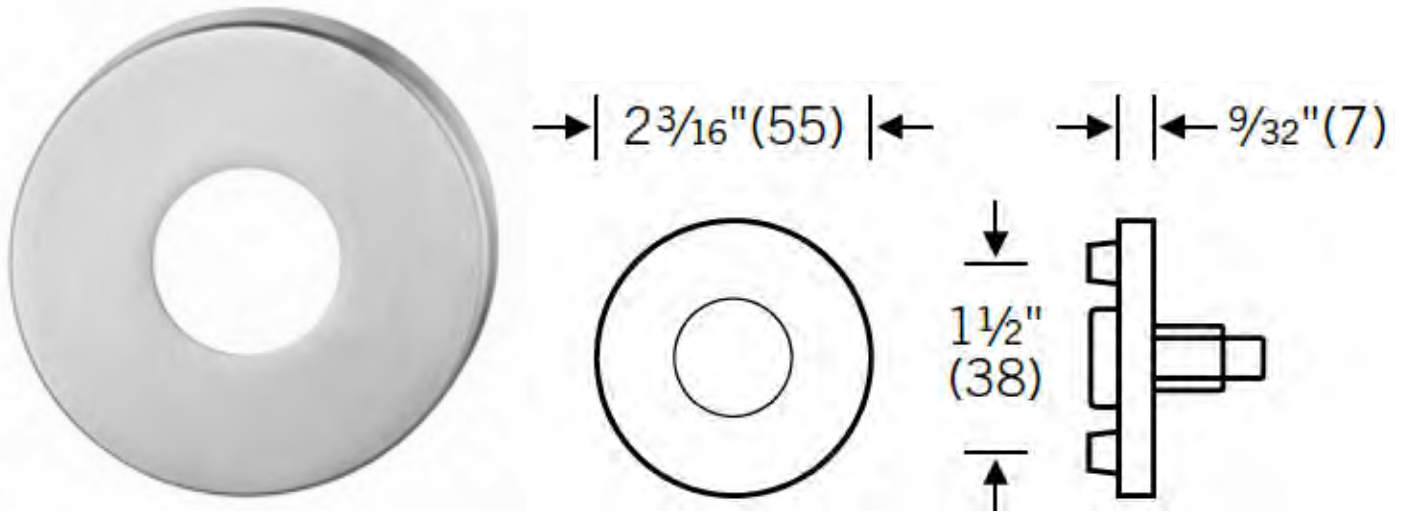
Rose for Lever: 12.110F 55 mm diameter All Parts Stainless Steel
