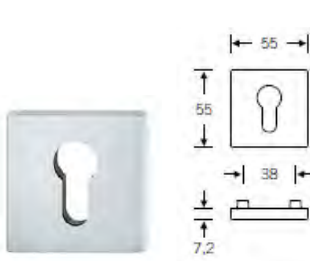
Square Key Rose #12.1704
