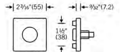
Stainless steel rose square, pair 55 x 55 mm or 2 3/16 inch Clip on style with inner rose Screws invisible
