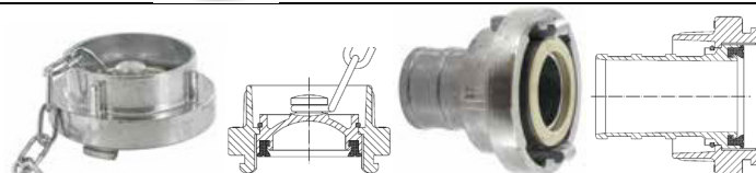
#91.052 Dustcover Storz N-52 (Brass or Aluminum) #91.066 Dustcover Storz N-66 (Brass or Aluminum) #91.1431 Storz coupling w. hose barb N-52 to 1 1/2" hose #91.1436 Storz coupling w. hose barb N-66 to 1 1/2" hose
