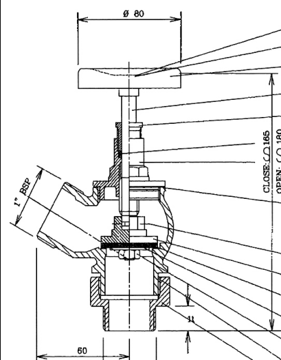
#91.075 Valve 1 inch showing with Stainless Steel Camlock Coupling & cap Steel powder coated turning wheel Thread: 1" BSP. Valve chrome plated brass
