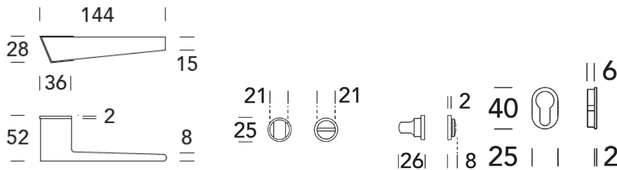
LEVER 15.0922 "WONDER" with roses 14.3713
