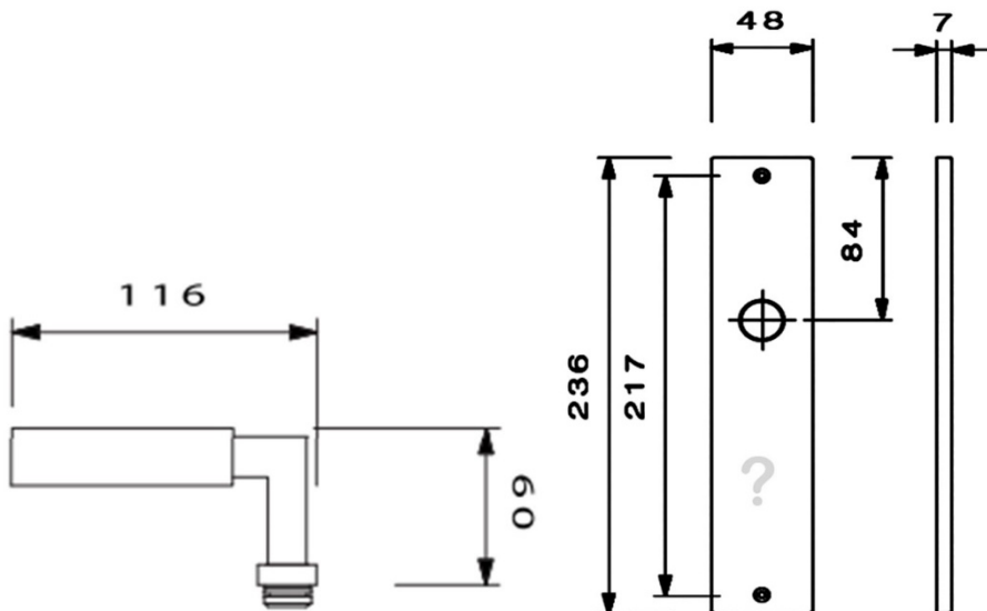
LEVER #14.964.266 set with escutcheon "BAUHAUS" Escutcheon #14.J964 236 x 48 x 7 mm Polished Chrome Plated Brass Plated.
