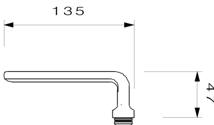
LEVER #13.J3685 "PURE QUATTRO" ROSE #13.J371 Polished chrome plated brass
