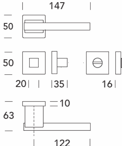
With square rose 50x50 mm; all functions available
