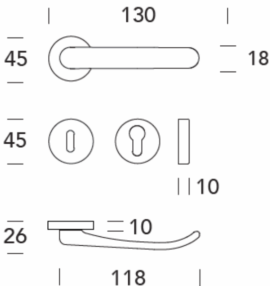
LEVER: 15.0076.106 "EXTRA BASSA" - NARROW STYLE STANDS OFF ONLY 26 MM OR 1 INCH FROM SURFACE
