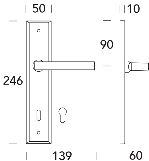
Escutcheon Lazer #15.MP130. dimensions: 50 x 246 x 10
