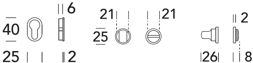
Cylinder Key Rose and Privacy thumb-turn- indicator
