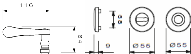
LEVER #13.J9015 "SCHONBRUNN" ESCUTCHEON #13.J51
