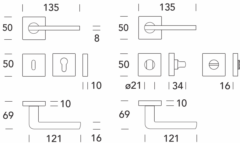
Drawings showing dimensions square roses 50 x 50 mm All Functions (Passage, Privacy and Entry) available
