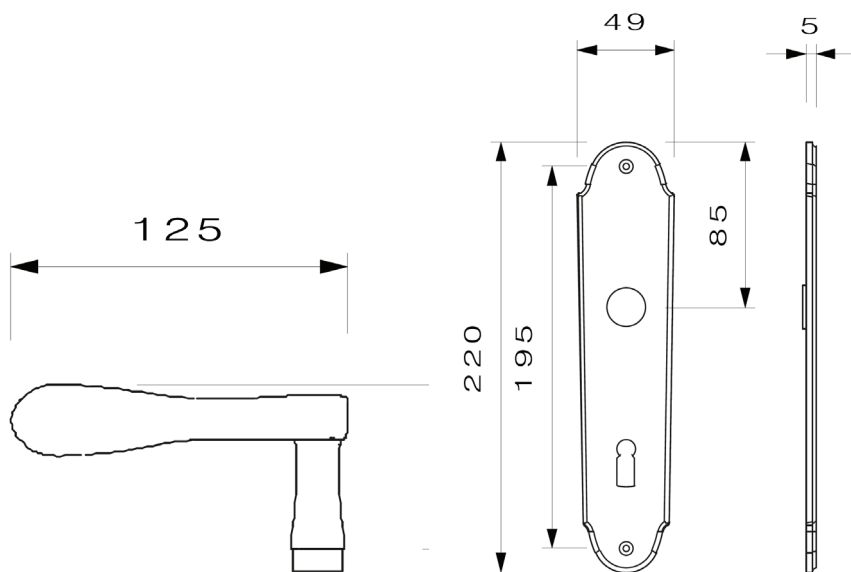
Lever Belvedere #13.J988 with Escutcheon 13.J988
