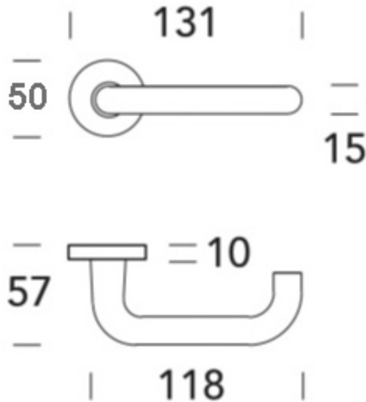
SHIPS LEVER: 15.0130 "ELENA"
