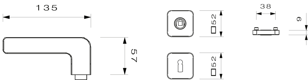
55 mm backset Doorthickness: 1 ½ inch
