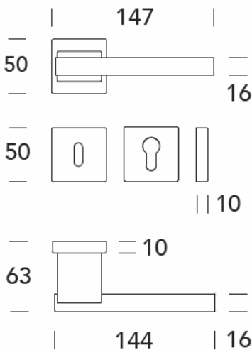
With square rose 50x50 mm; all functions available
