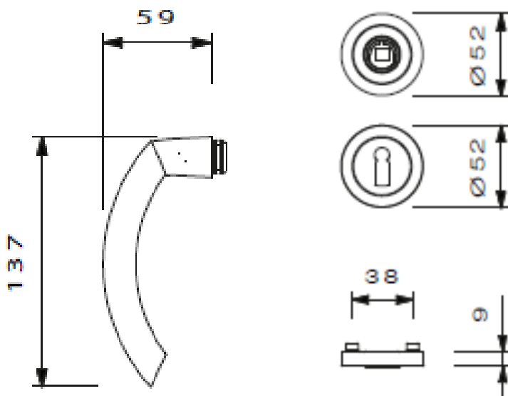
ROSE LEVER #13.J9613 "AVANCE" #13.J361 (Minor different from picture shown) Polished Lacquered Brass
