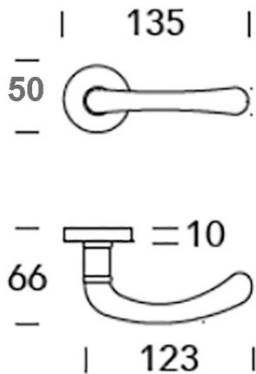
SHIPS LEVER: 15.0166 "MONIA 037"
