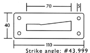
Strike angle: #43.999
