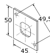
Set: Hatch fastener with mounting plate and cam #43.295 Mounting plate
