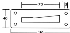
Angle strike for straight cam 43.999
