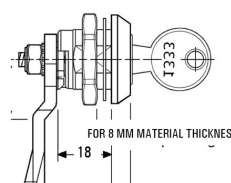
#43.687K Key operated 18 mm body.
