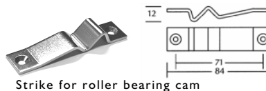
Strike for roller bearing cam
