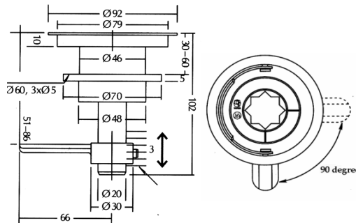
#43.954 Hatch fastener with lift ring
