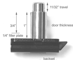
#24.080 Cabinet pull; 92x37x22mm. 29.2020 series Push latch Black body. #29.2025 Body + filler plate 1/4" thick. Aluminum color body #29.2025
