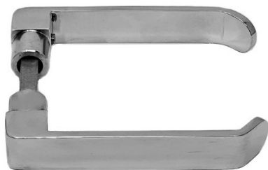
Lever #12.555; 115 mm long; stand off 25 mm with standard plate; 20 mm wide This picture: showing with glass door mechanism #82.511.18
